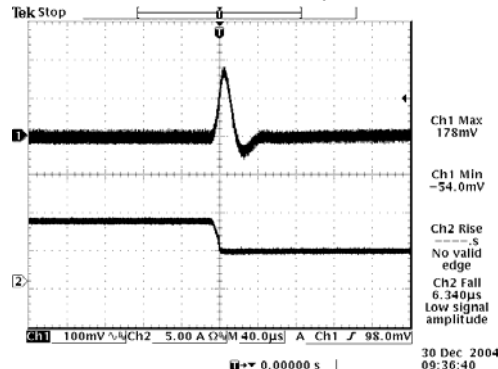
100% to 50% load 12 Vdc Input 1.8 Vdc Output
